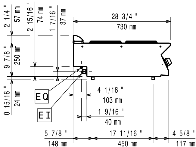
Lateral
